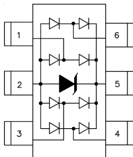
SOT-23 6L (Top View)
